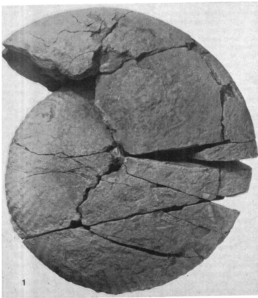
Fig. 1. Mayaites (Araucanites) stipanicii West. et Rice., subgen. et sp. nov., holotype, complete specimen, lateral view, \times 0.75 (M.I.P. 12240). Plicatilis (? U. Cordatum) Zone, locality XI, Aguada de Campos, Sierra de Reyes.
