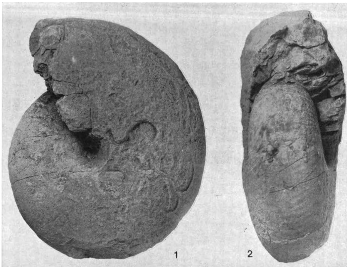
Figs. 1-2. Mayaites (Araucanites) mutai West. et Ricc., subgen. et sp. nov., holotype, complete specimen, lateral and ventral views. \times 1 (MLP 12247). Plicatilis (? U. Cordatum ) Zone, Aguada de la Mula, Sierra de Reyes.
