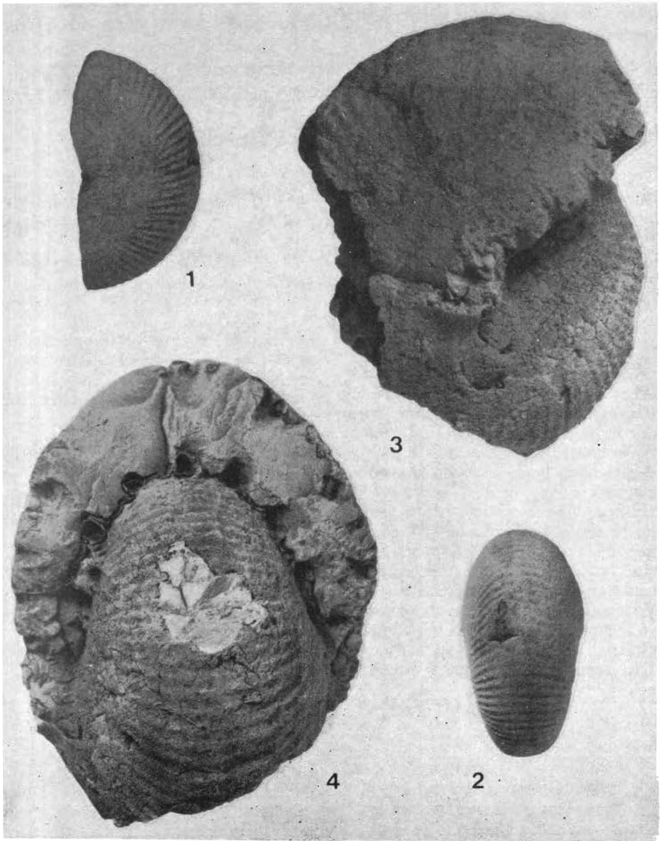
Figs. 1-2. Mayaites (Araucanites) reyesi West. et Rice., subgen. et sp. nov., juvenile phragmocone, lateral and ventral views, \times 1 (MLP 12243). Plicatilis (? Cordatum) Zone, Aguada de la Mula, Sierra de Reyes: 3-4, Mayaites (Araucanites) sp. nov. ? 1, damaged adult phragmocone, lateral and ventral views, \times 1 (MLP 12246). Same age and locality.
