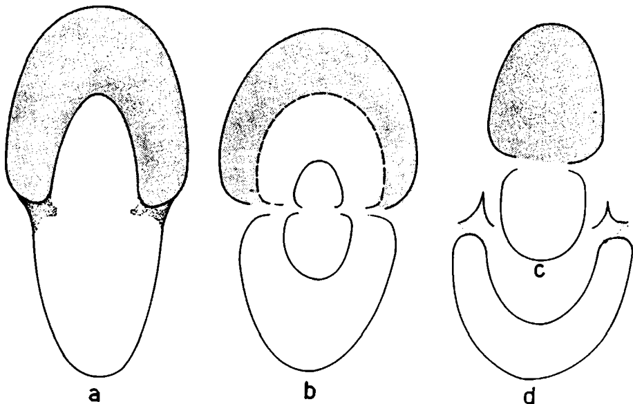
Fig. 4. — Cross-sections through phragmocone (white) and body chamber (grey) of: a , Mayaites (Araucanites) stipanici sp. nov., holotype (MLP 12240); b , M. (A.) reyesi sp. nov., holotype and paratypes (MLP 12241-43); c , M. (A.) mulai sp. nov., holotype (MLP 12247) and d , M. (A.) sp. nov. ? 1 (MLP 12246). c. \times 12 .
