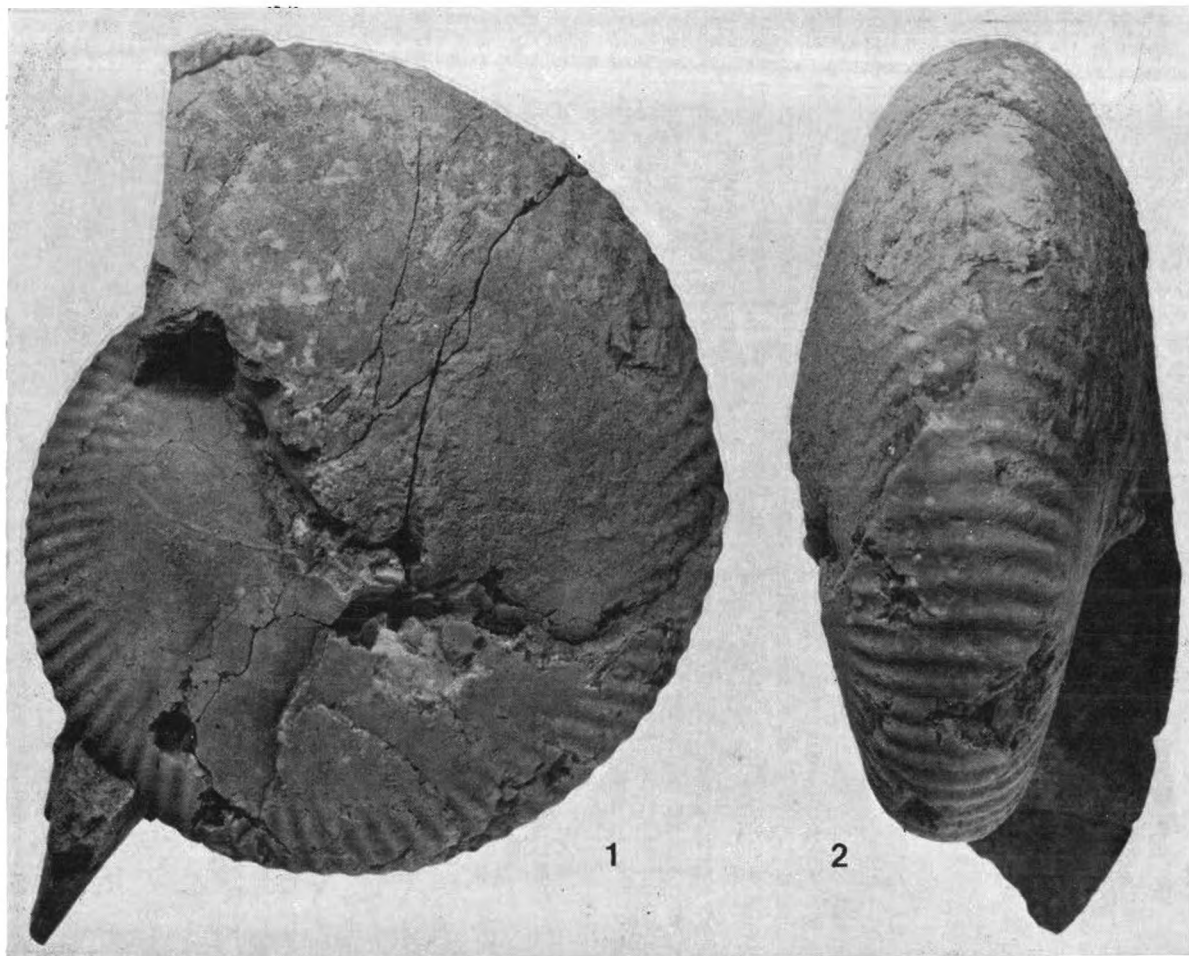
Figs. 1-2. Mayaites (Araucanites) stipanicici West. et Ricc., subgen. et sp. nov., body chamber removed, lateral and ventral views, \times 1 (MLP 12240). Plicatilis (? U. Cordatum) Zone, locality XI. Aguada de Campos, Sierra de Reyes.
