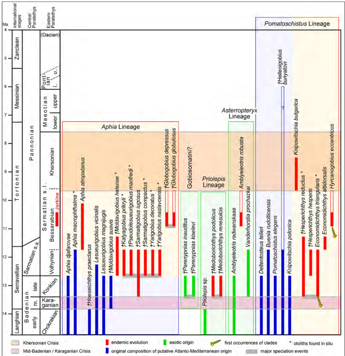
Fig. 21 - Range chart of otolith-based taxa of the Aphia , Priolepis , Asterropteryx and Pomatoschistus lineages and the Gobiosomatini in the Paratethys from Middle Miocene to Early Pliocene. Blue bars indicate taxa of Atlanto-Mediterranean origin and shared with time-equivalent occurrences in other European basins; red bars indicate putative endemic taxa in the Paratethys; green bars indicate non-indigenous lineages in European seas; open bars indicate possible range extensions.
