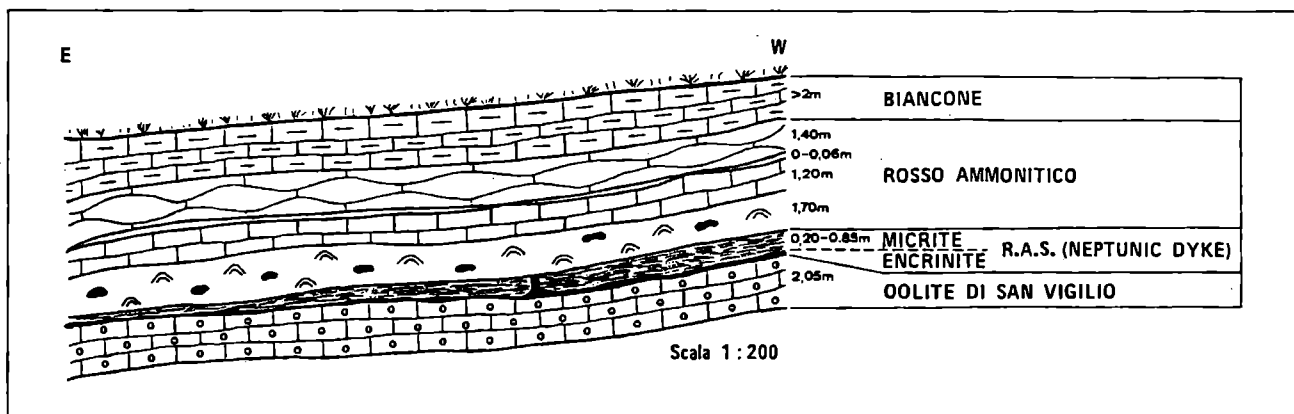
Fig. 1 Sketch of the northern part of the Western Lessinian Mountains (VR).
