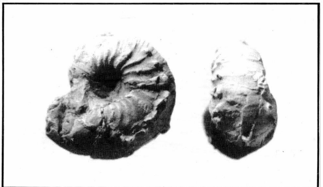
Fig. 2 - Sutneria platynota (Reinecke), Loc. Ambrosi near Breonio, 2x, Lower Kimmeridgian (first documentation of the species from Italy), Lateral and ventral view.
