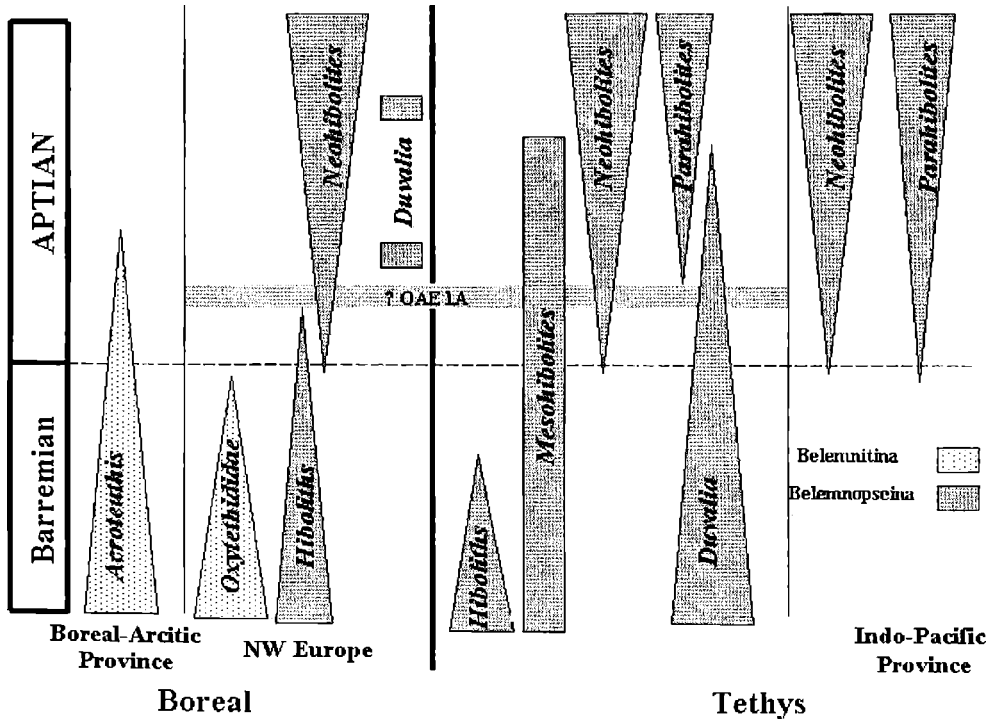
Fig. 3: Global range of various belemnite taxa from the Barremian-Aptian boundary (after Mutterlose 1998).
